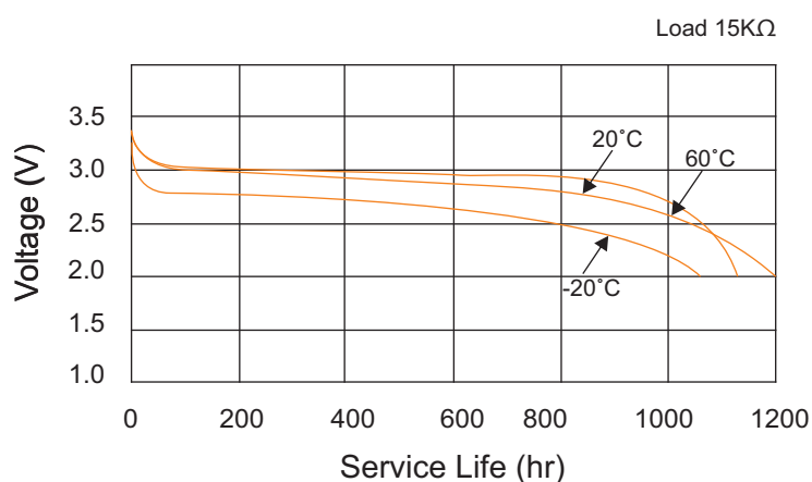
Temperature Characteristics
