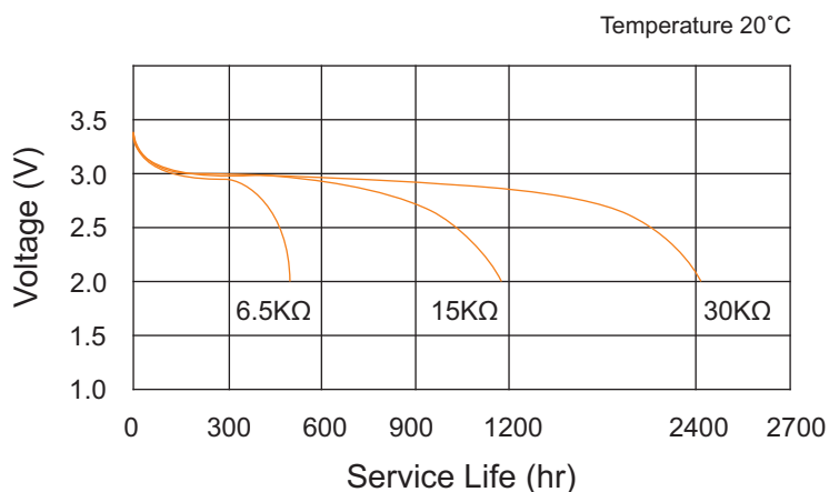
Discharge Characteristics
